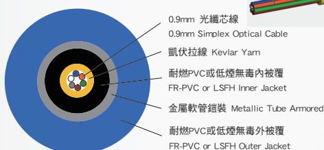
裸光纖 Bare Fiber PVC被覆 PVC Tight Buffer
